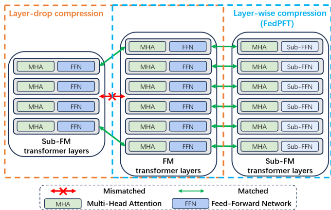
(a) Two types of proxy sub-FM construction
